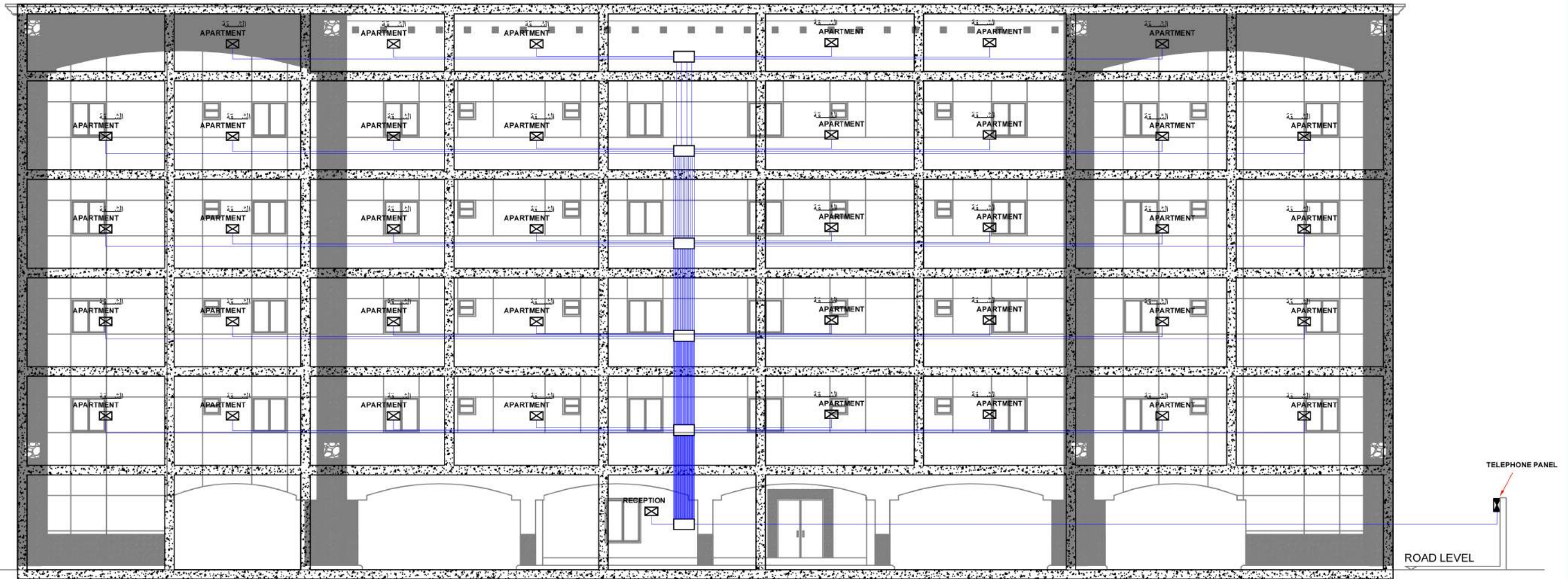
FRONT SIDE ELEVATION
